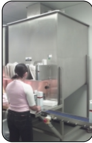
Vertical Transfer Lift from Cleanroom and Packing Station
